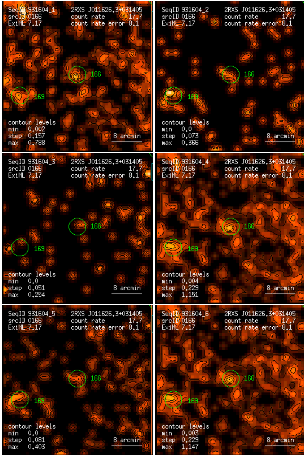
Figure 166: RASS 931604: detection 0166: band rate images, Gaussian filter: (1) PSPC channels 11 – 41, (2) 52 – 90, (3) 91 – 201, (4) 11 – 235, (5) 52 – 201, (6) 11 – 201. Broad band rates in counts/ks. Band rate contour levels in counts/ks/arcmin 2 .
