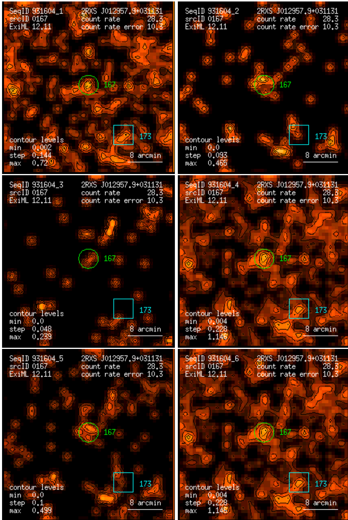
Figure 167: RASS 931604: detection 0167: band rate images, Gaussian filter: (1) PSPC channels 11 – 41, (2) 52 – 90, (3) 91 – 201, (4) 11 – 235, (5) 52 – 201, (6) 11 – 201. Broad band rates in counts/ks. Band rate contour levels in counts/ks/arcmin 2 .
