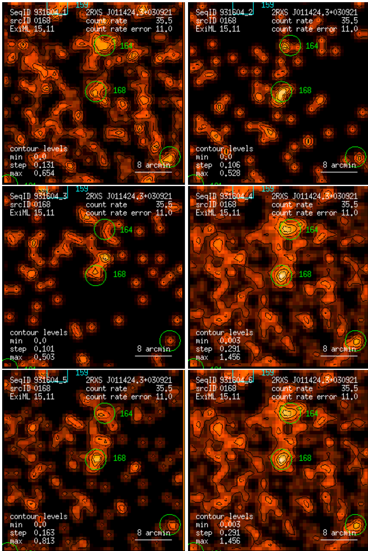
Figure 168: RASS 931604: detection 0168: band rate images, Gaussian filter: (1) PSPC channels 11 – 41, (2) 52 – 90, (3) 91 – 201, (4) 11 – 235, (5) 52 – 201, (6) 11 – 201. Broad band rates in counts/ks. Band rate contour levels in counts/ks/arcmin 2 .
