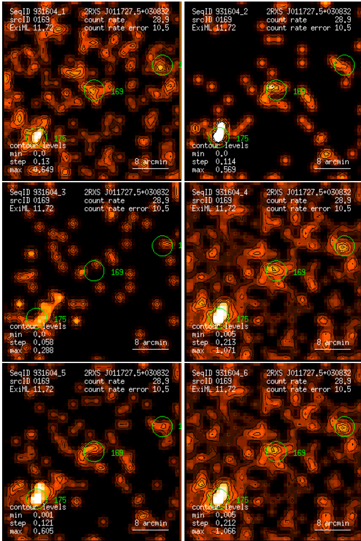
Figure 169: RASS 931604: detection 0169: band rate images, Gaussian filter: (1) PSPC channels 11 – 41, (2) 52 – 90, (3) 91 – 201, (4) 11 – 235, (5) 52 – 201, (6) 11 – 201. Broad band rates in counts/ks. Band rate contour levels in counts/ks/arcmin 2 .
