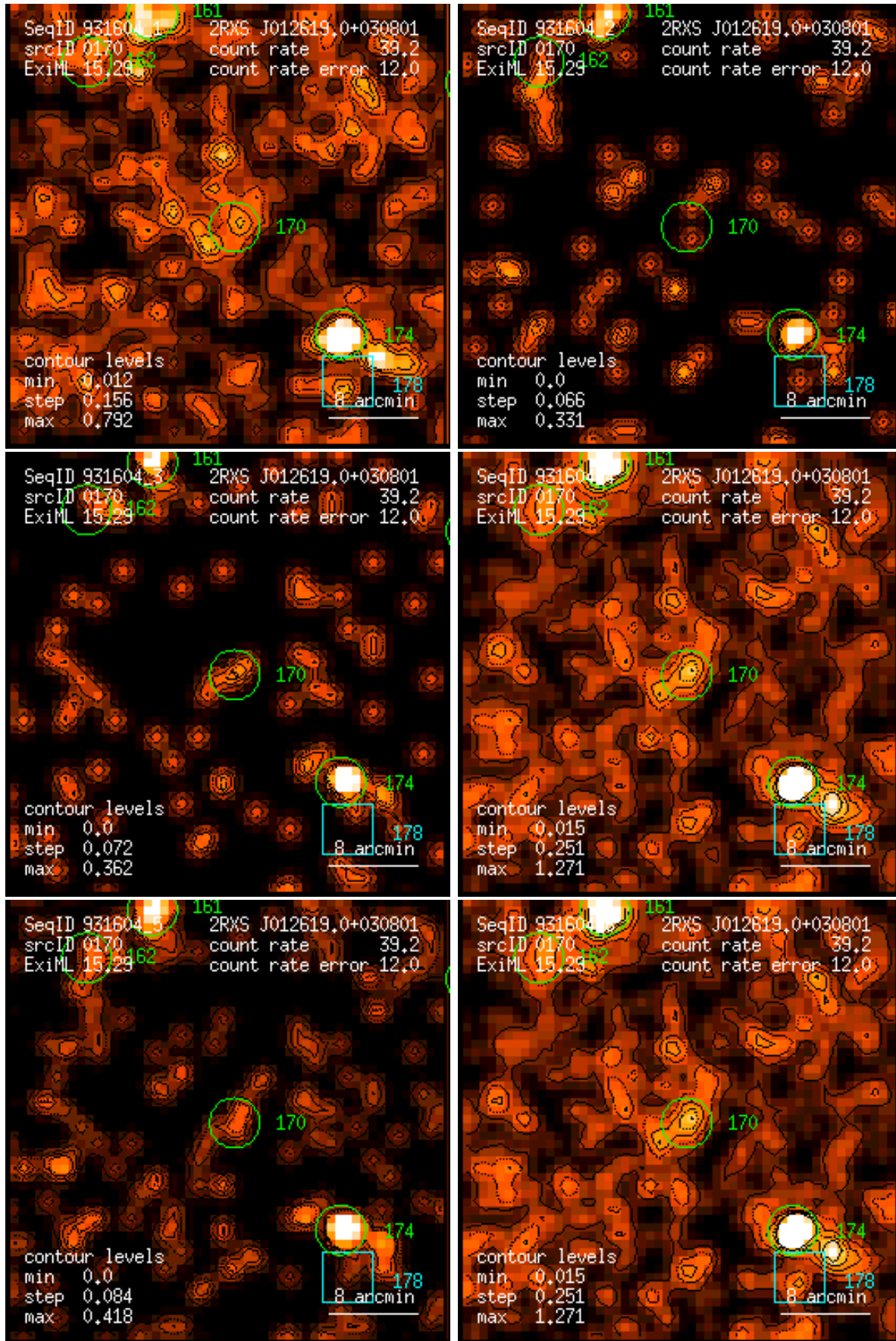
Figure 170: RASS 931604: detection 0170: band rate images, Gaussian filter: (1) PSPC channels 11 – 41, (2) 52 – 90, (3) 91 – 201, (4) 11 – 235, (5) 52 – 201, (6) 11 – 201. Broad band rates in counts/ks. Band rate contour levels in counts/ks/arcmin 2 .
