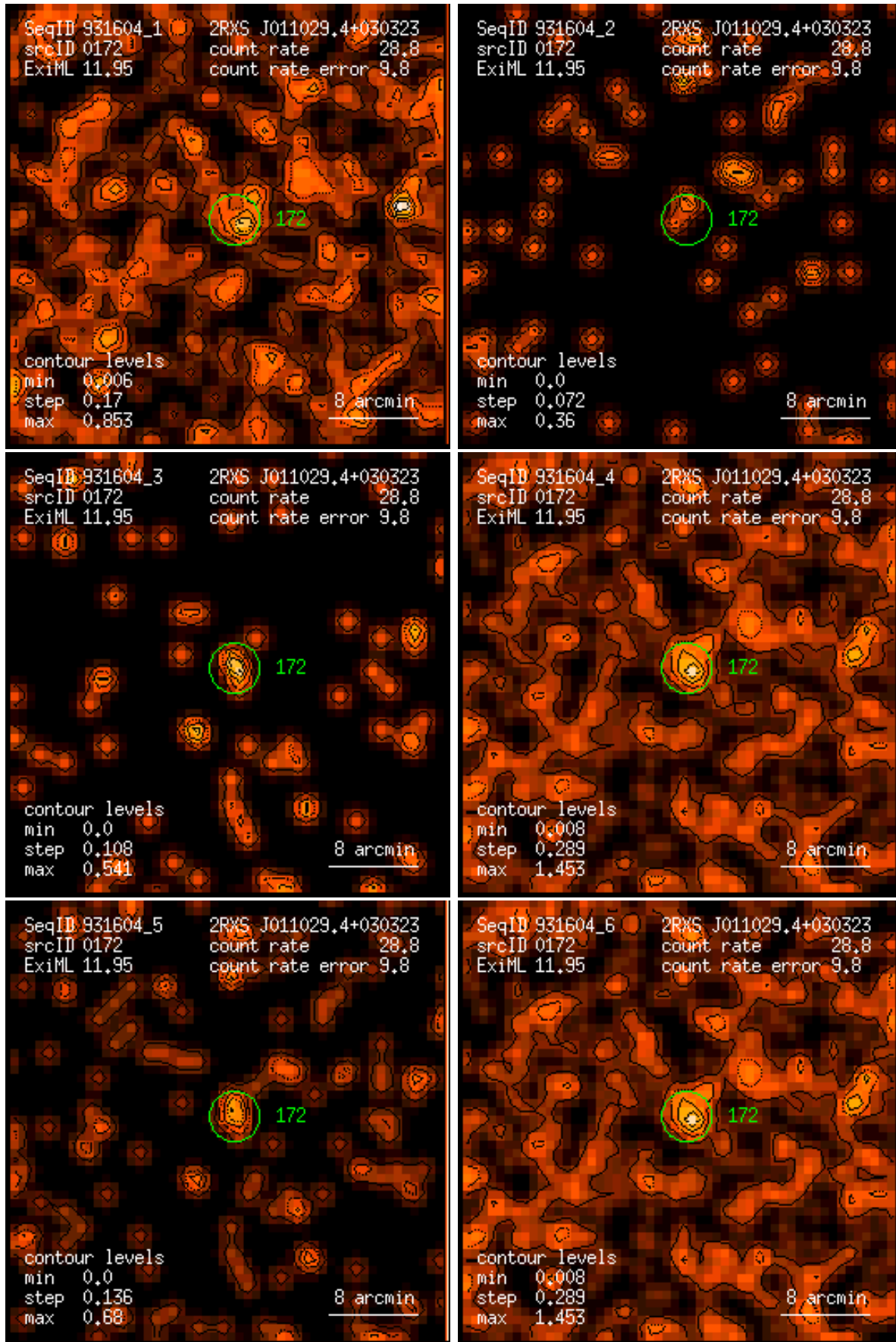
Figure 172: RASS 931604: detection 0172: band rate images, Gaussian filter: (1) PSPC channels 11 – 41, (2) 52 – 90, (3) 91 – 201, (4) 11 – 235, (5) 52 – 201, (6) 11 – 201. Broad band rates in counts/ks. Band rate contour levels in counts/ks/arcmin 2 .
