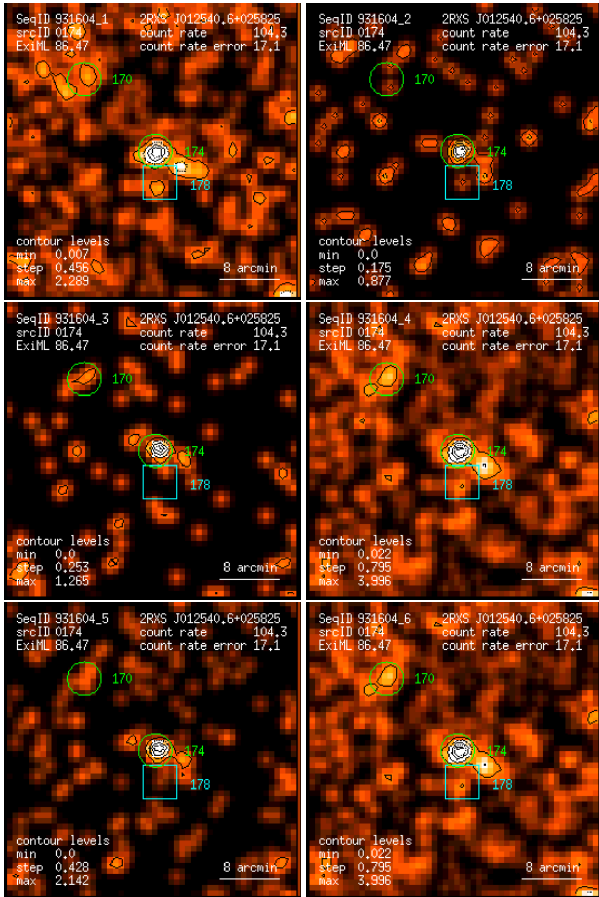
Figure 174: RASS 931604: detection 0174: band rate images, Gaussian filter: (1) PSPC channels 11 – 41, (2) 52 – 90, (3) 91 – 201, (4) 11 – 235, (5) 52 – 201, (6) 11 – 201. Broad band rates in counts/ks. Band rate contour levels in counts/ks/arcmin 2 .
