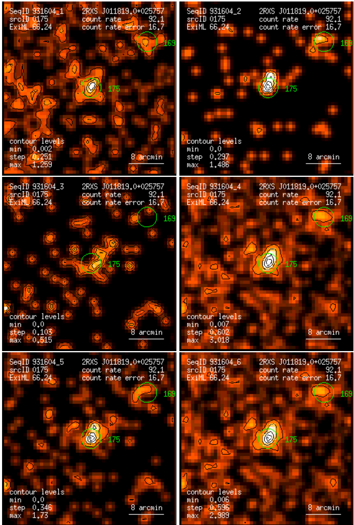
Figure 175: RASS 931604: detection 0175: band rate images, Gaussian filter: (1) PSPC channels 11 – 41, (2) 52 – 90, (3) 91 – 201, (4) 11 – 235, (5) 52 – 201, (6) 11 – 201. Broad band rates in counts/ks. Band rate contour levels in counts/ks/arcmin 2 .
