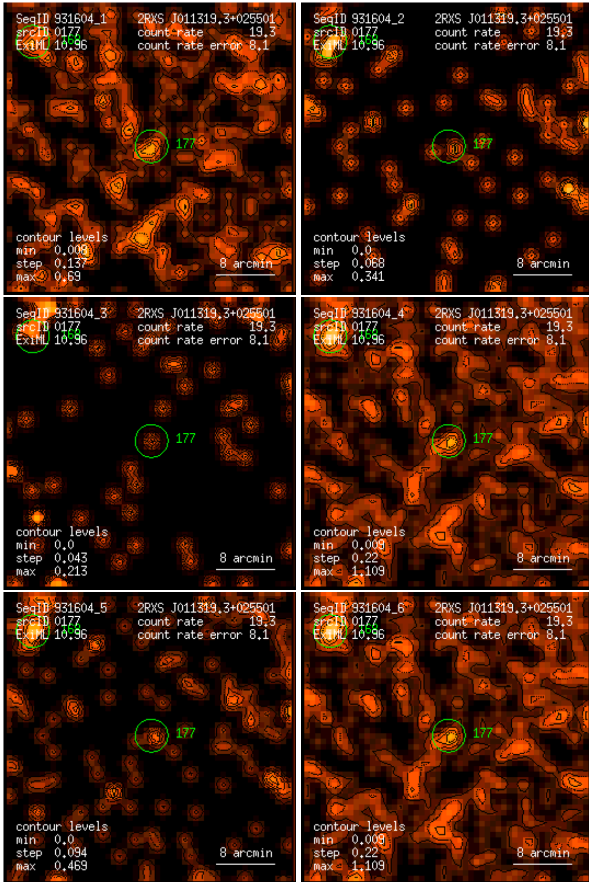
Figure 177: RASS 931604: detection 0177: band rate images, Gaussian filter: (1) PSPC channels 11 – 41, (2) 52 – 90, (3) 91 – 201, (4) 11 – 235, (5) 52 – 201, (6) 11 – 201. Broad band rates in counts/ks. Band rate contour levels in counts/ks/arcmin 2 .
