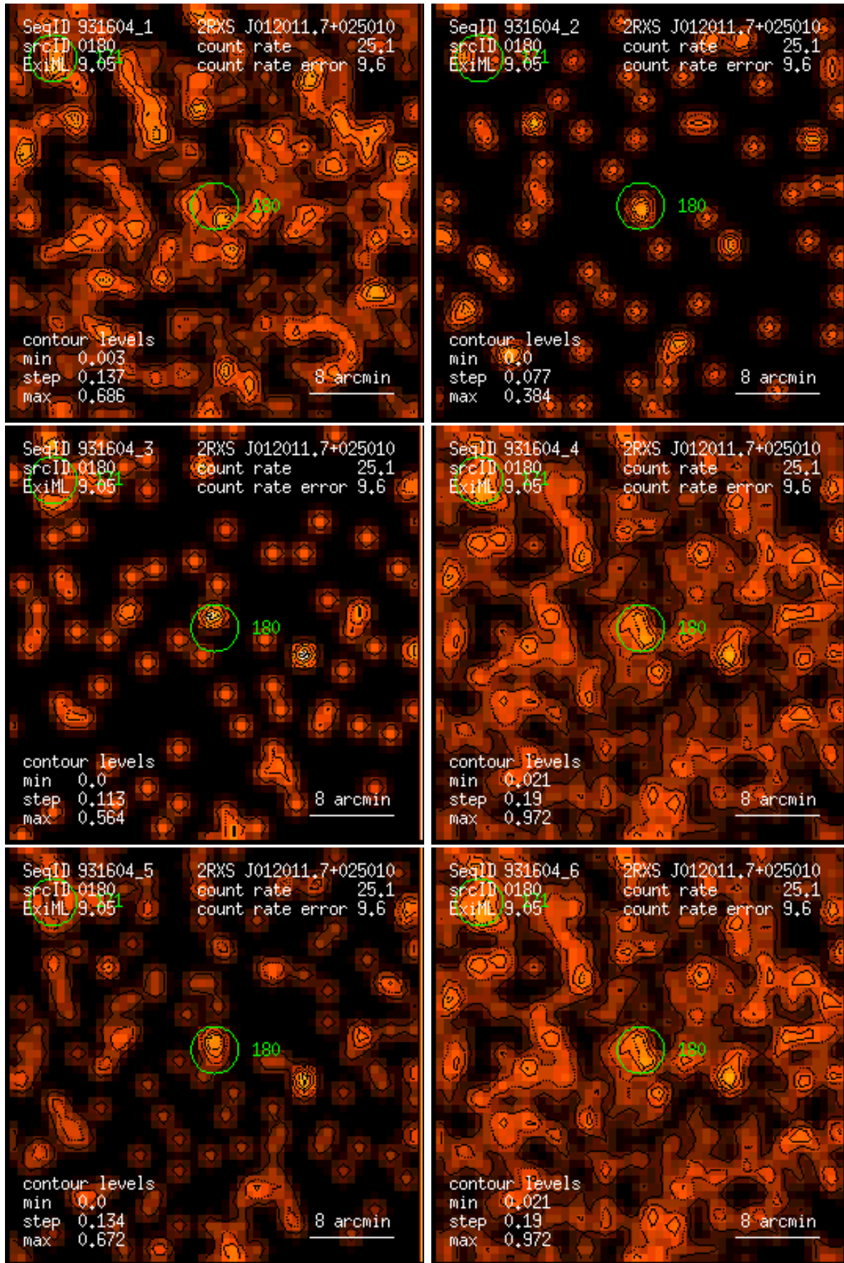
Figure 180: RASS 931604: detection 0180: band rate images, Gaussian filter: (1) PSPC channels 11 – 41, (2) 52 – 90, (3) 91 – 201, (4) 11 – 235, (5) 52 – 201, (6) 11 – 201. Broad band rates in counts/ks. Band rate contour levels in counts/ks/arcmin 2 .
