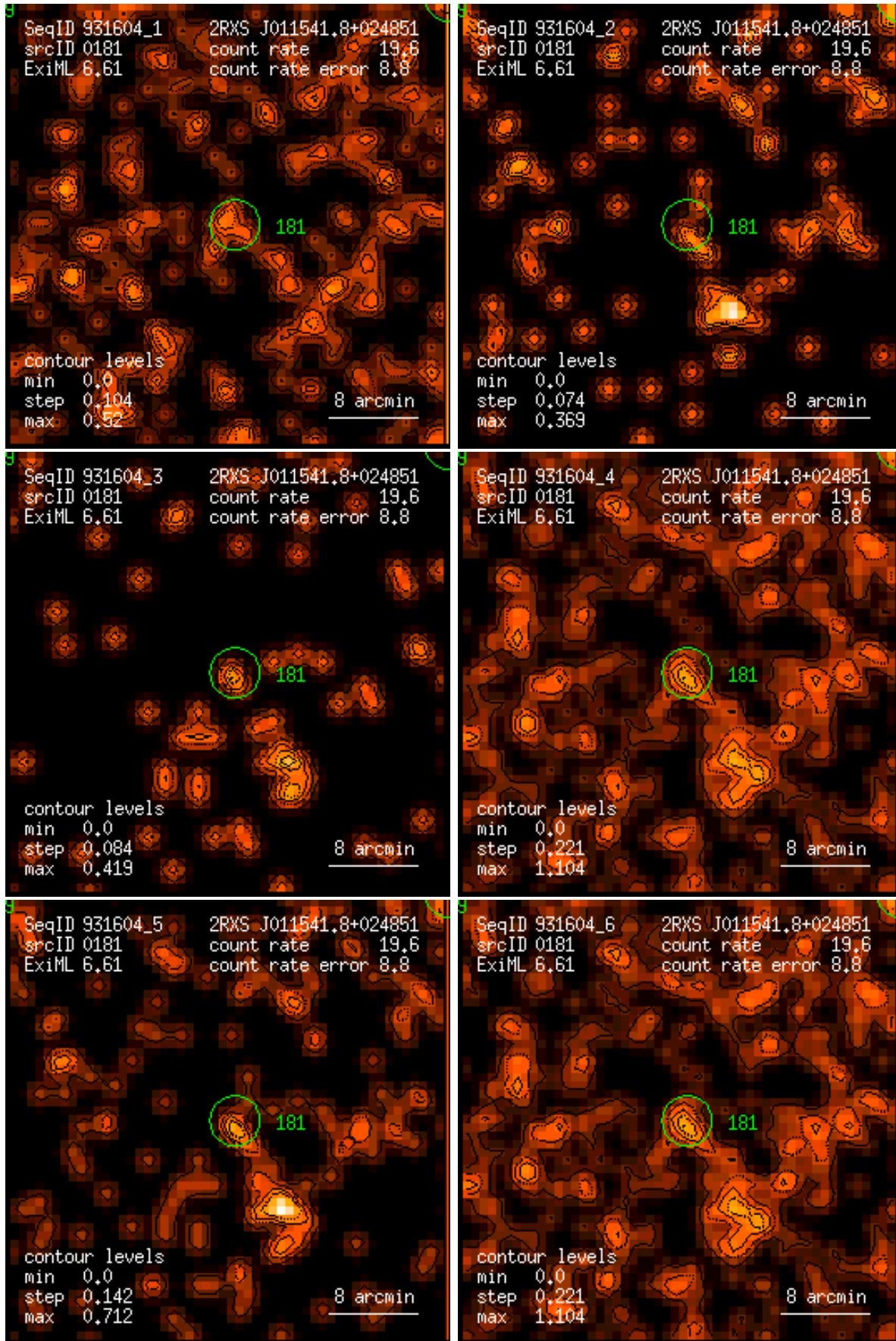
Figure 181: RASS 931604: detection 0181: band rate images, Gaussian filter: (1) PSPC channels 11 – 41, (2) 52 – 90, (3) 91 – 201, (4) 11 – 235, (5) 52 – 201, (6) 11 – 201. Broad band rates in counts/ks. Band rate contour levels in counts/ks/arcmin 2 .
