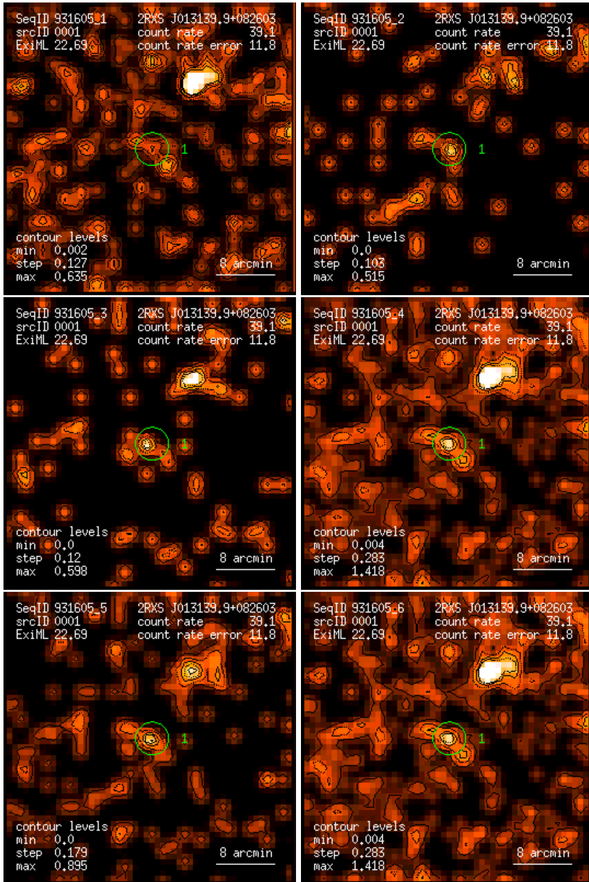
Figure 1: RASS 931605: detection 0001: band rate images, Gaussian filter: (1) PSPC channels 11 – 41, (2) 52 – 90, (3) 91 – 201, (4) 11 – 235, (5) 52 – 201, (6) 11 – 201. Broad band rates in counts/ks. Band rate contour levels in counts/ks/arcmin 2 .
