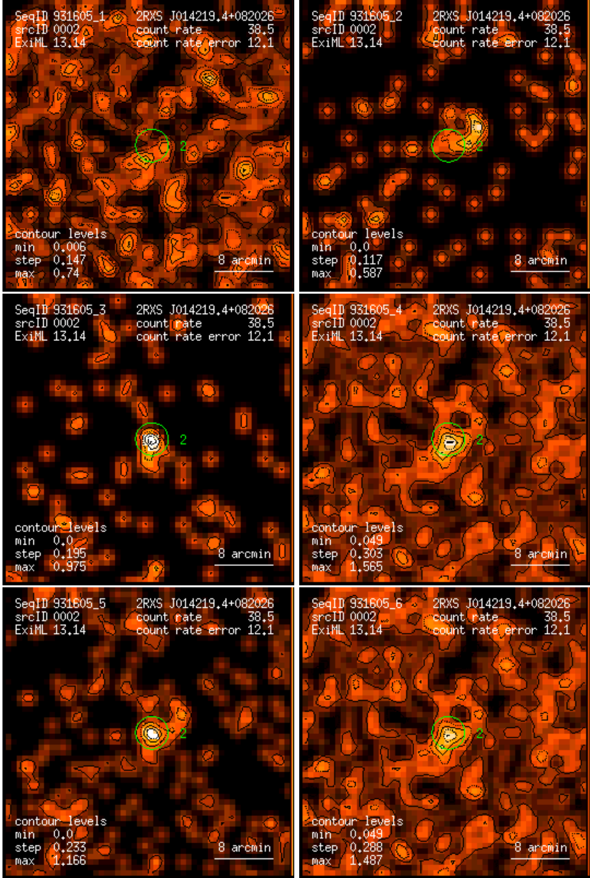
Figure 2: RASS 931605: detection 0002: band rate images, Gaussian filter: (1) PSPC channels 11 – 41, (2) 52 – 90, (3) 91 – 201, (4) 11 – 235, (5) 52 – 201, (6) 11 – 201. Broad band rates in counts/ks. Band rate contour levels in counts/ks/arcmin 2 .
