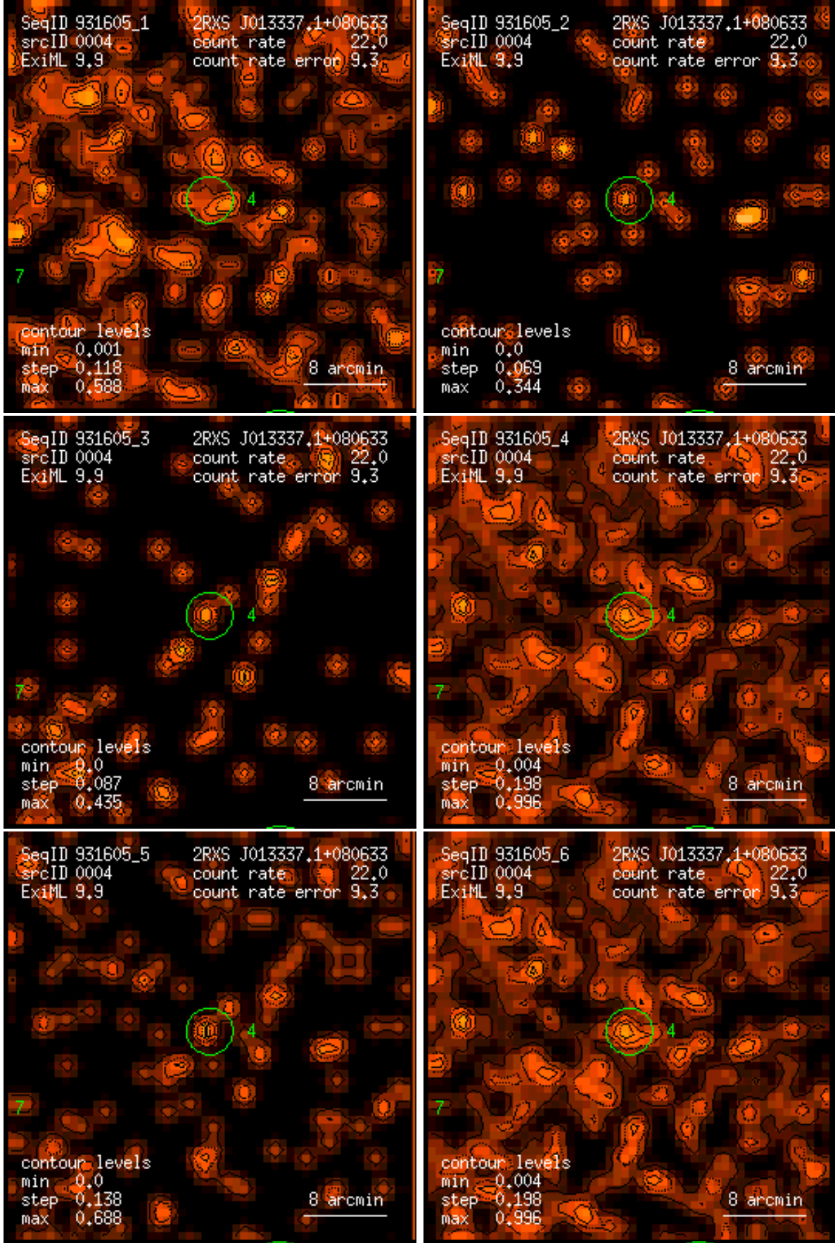
Figure 4: RASS 931605: detection 0004: band rate images, Gaussian filter: (1) PSPC channels 11 – 41, (2) 52 – 90, (3) 91 – 201, (4) 11 – 235, (5) 52 – 201, (6) 11 – 201. Broad band rates in counts/ks. Band rate contour levels in counts/ks/arcmin 2 .
