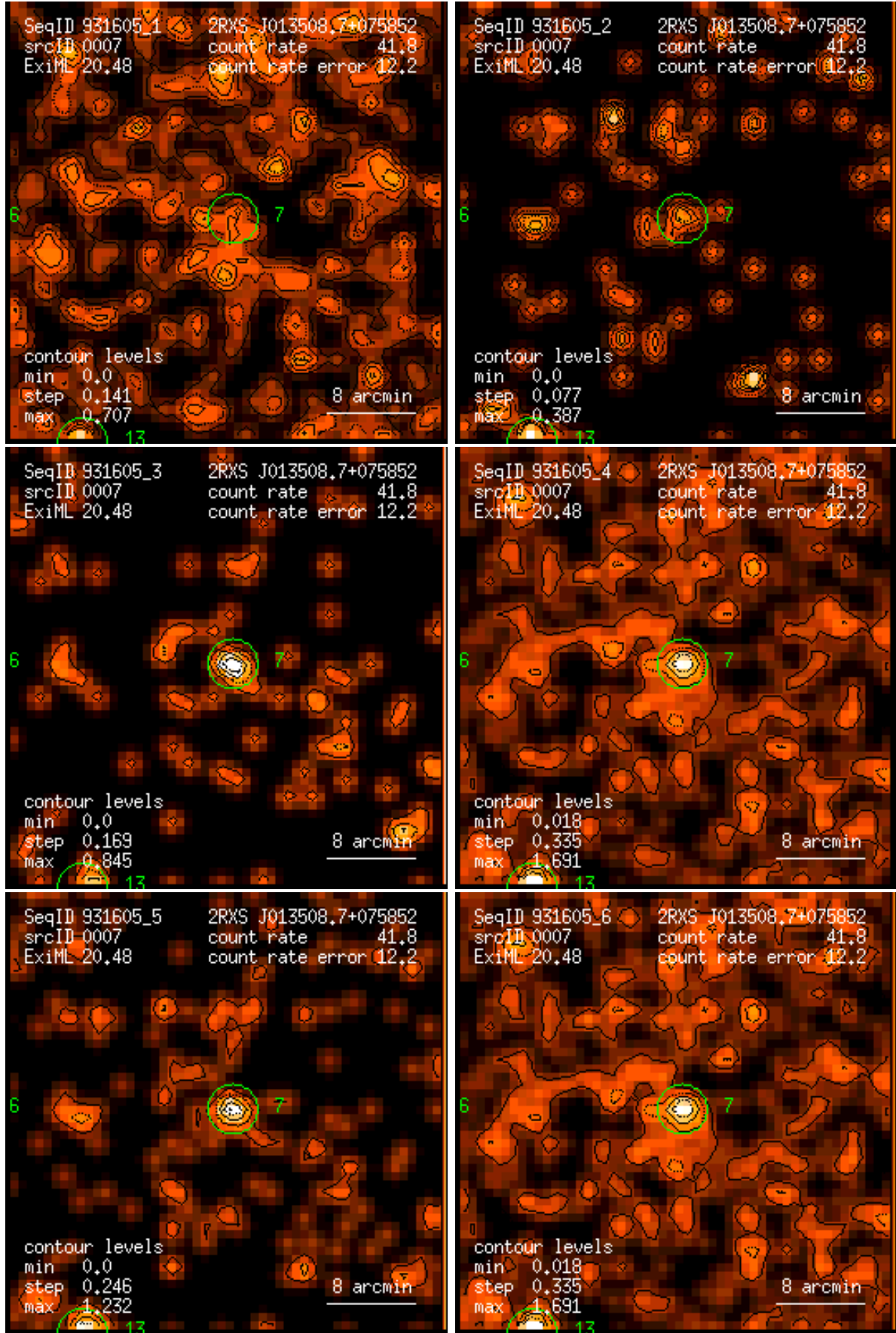
Figure 7: RASS 931605: detection 0007: band rate images, Gaussian filter: (1) PSPC channels 11 – 41, (2) 52 – 90, (3) 91 – 201, (4) 11 – 235, (5) 52 – 201, (6) 11 – 201. Broad band rates in counts/ks. Band rate contour levels in counts/ks/arcmin 2 .
