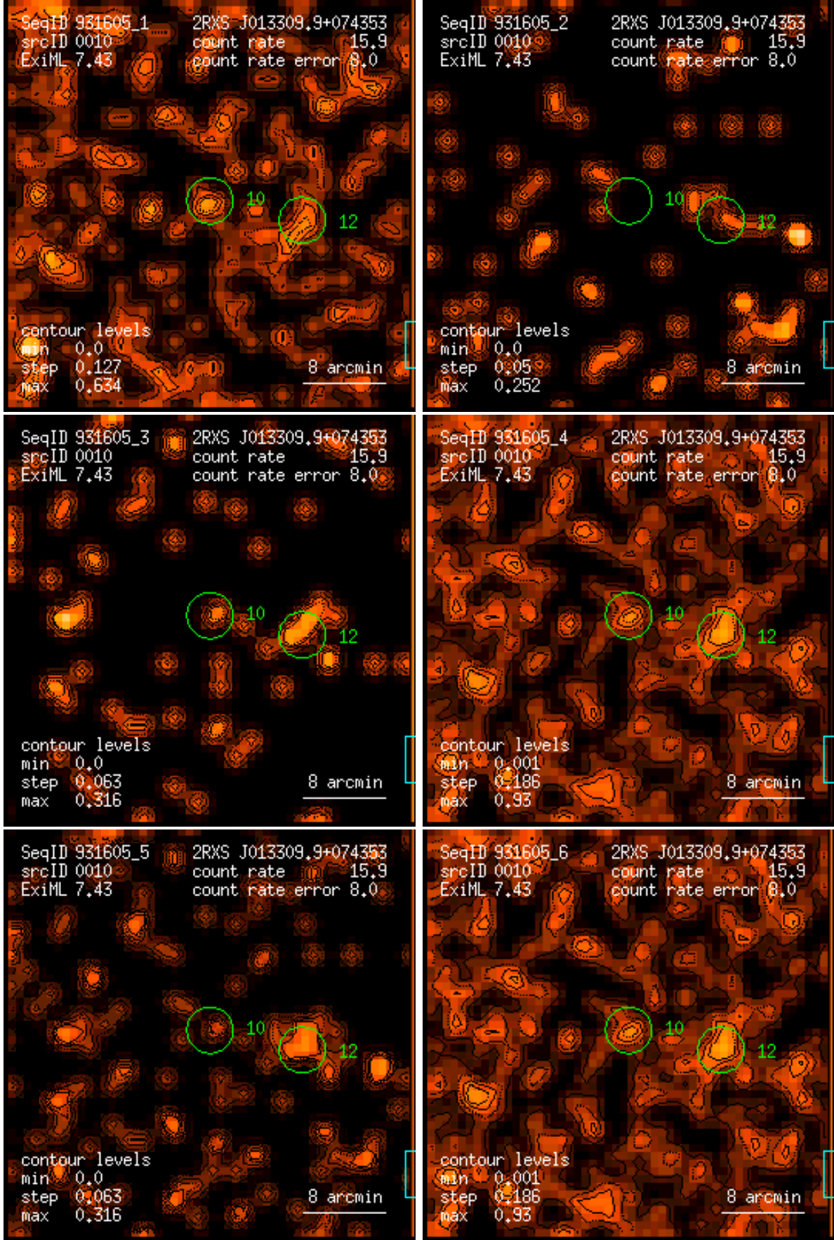
Figure 10: RASS 931605: detection 0010: band rate images, Gaussian filter: (1) PSPC channels 11 – 41, (2) 52 – 90, (3) 91 – 201, (4) 11 – 235, (5) 52 – 201, (6) 11 – 201. Broad band rates in counts/ks. Band rate contour levels in counts/ks/arcmin 2 .
