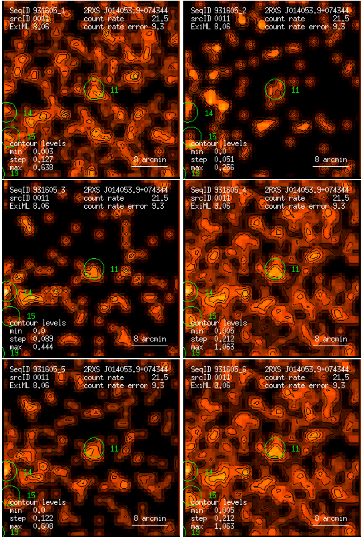
Figure 11: RASS 931605: detection 0011: band rate images, Gaussian filter: (1) PSPC channels 11 – 41, (2) 52 – 90, (3) 91 – 201, (4) 11 – 235, (5) 52 – 201, (6) 11 – 201. Broad band rates in counts/ks. Band rate contour levels in counts/ks/arcmin 2 .
