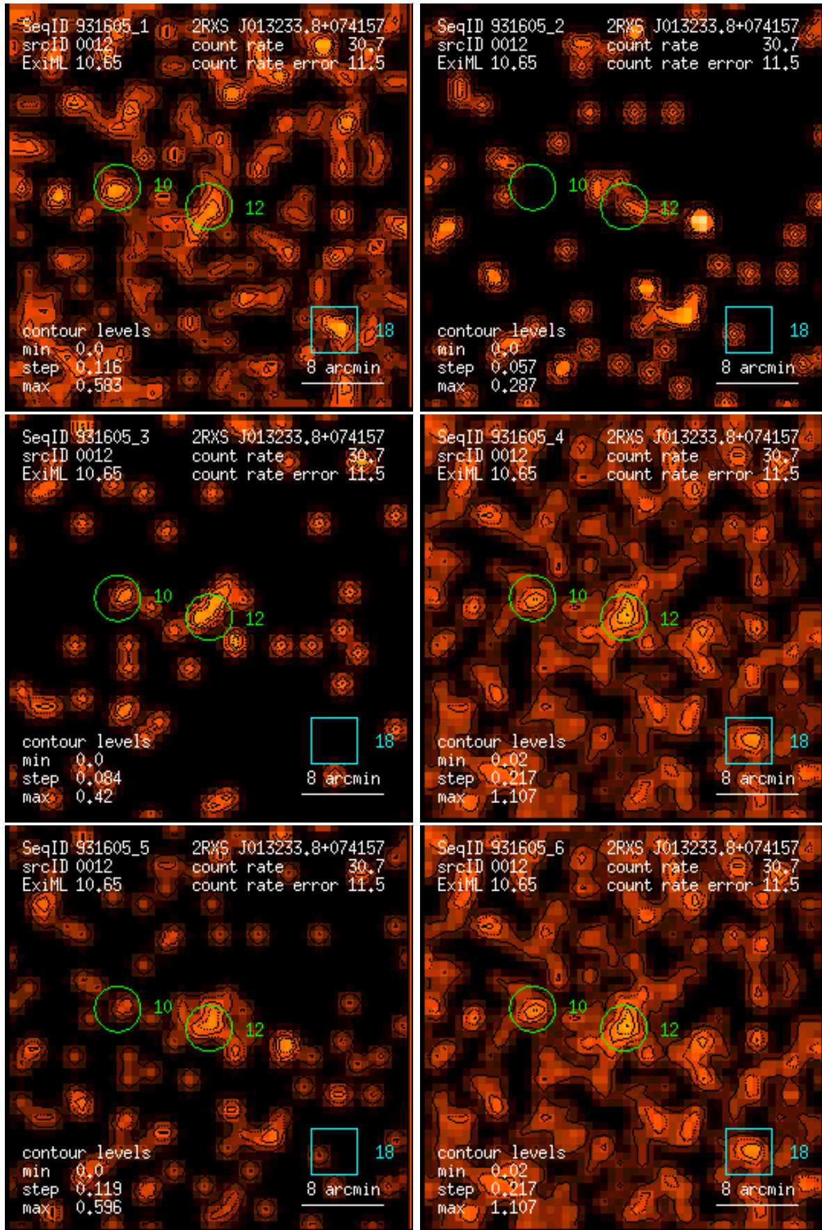
Figure 12: RASS 931605: detection 0012: band rate images, Gaussian filter: (1) PSPC channels 11 – 41, (2) 52 – 90, (3) 91 – 201, (4) 11 – 235, (5) 52 – 201, (6) 11 – 201. Broad band rates in counts/ks. Band rate contour levels in counts/ks/arcmin 2 .
