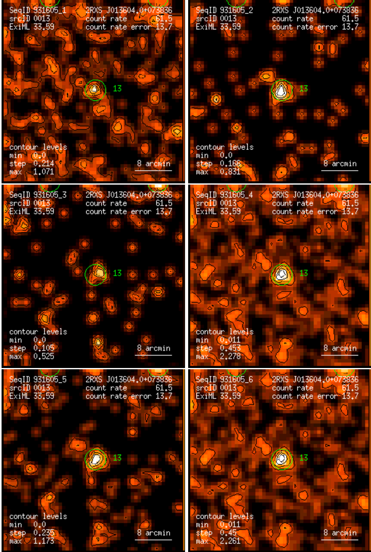
Figure 13: RASS 931605: detection 0013: band rate images, Gaussian filter: (1) PSPC channels 11 – 41, (2) 52 – 90, (3) 91 – 201, (4) 11 – 235, (5) 52 – 201, (6) 11 – 201. Broad band rates in counts/ks. Band rate contour levels in counts/ks/arcmin 2 .
