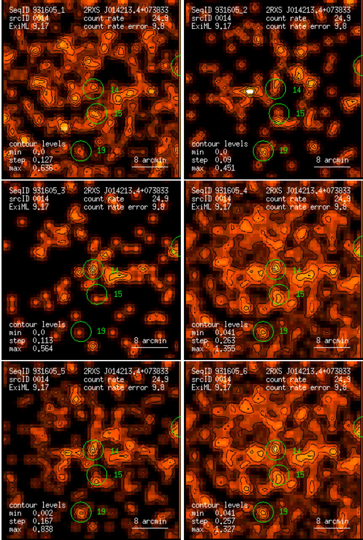
Figure 14: RASS 931605: detection 0014: band rate images, Gaussian filter: (1) PSPC channels 11 – 41, (2) 52 – 90, (3) 91 – 201, (4) 11 – 235, (5) 52 – 201, (6) 11 – 201. Broad band rates in counts/ks. Band rate contour levels in counts/ks/arcmin 2 .
