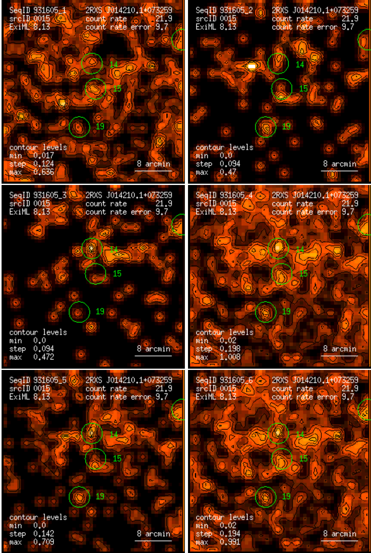
Figure 15: RASS 931605: detection 0015: band rate images, Gaussian filter: (1) PSPC channels 11 – 41, (2) 52 – 90, (3) 91 – 201, (4) 11 – 235, (5) 52 – 201, (6) 11 – 201. Broad band rates in counts/ks. Band rate contour levels in counts/ks/arcmin 2 .
