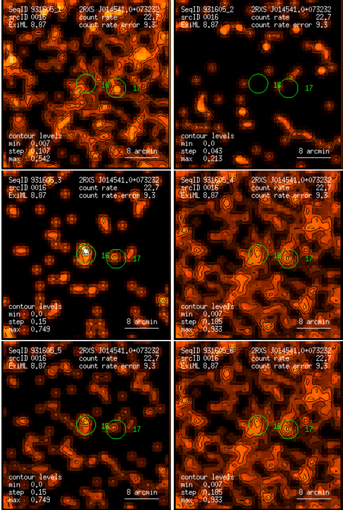
Figure 16: RASS 931605: detection 0016: band rate images, Gaussian filter: (1) PSPC channels 11 – 41, (2) 52 – 90, (3) 91 – 201, (4) 11 – 235, (5) 52 – 201, (6) 11 – 201. Broad band rates in counts/ks. Band rate contour levels in counts/ks/arcmin 2 .
