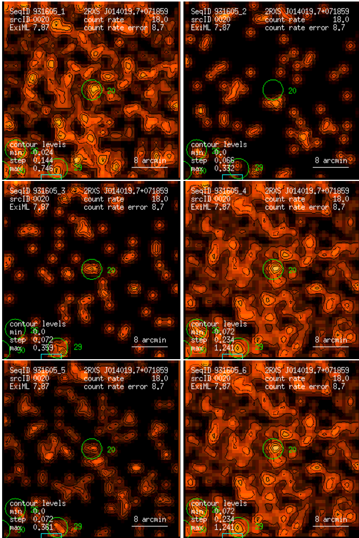
Figure 20: RASS 931605: detection 0020: band rate images, Gaussian filter: (1) PSPC channels 11 – 41, (2) 52 – 90, (3) 91 – 201, (4) 11 – 235, (5) 52 – 201, (6) 11 – 201. Broad band rates in counts/ks. Band rate contour levels in counts/ks/arcmin 2 .
