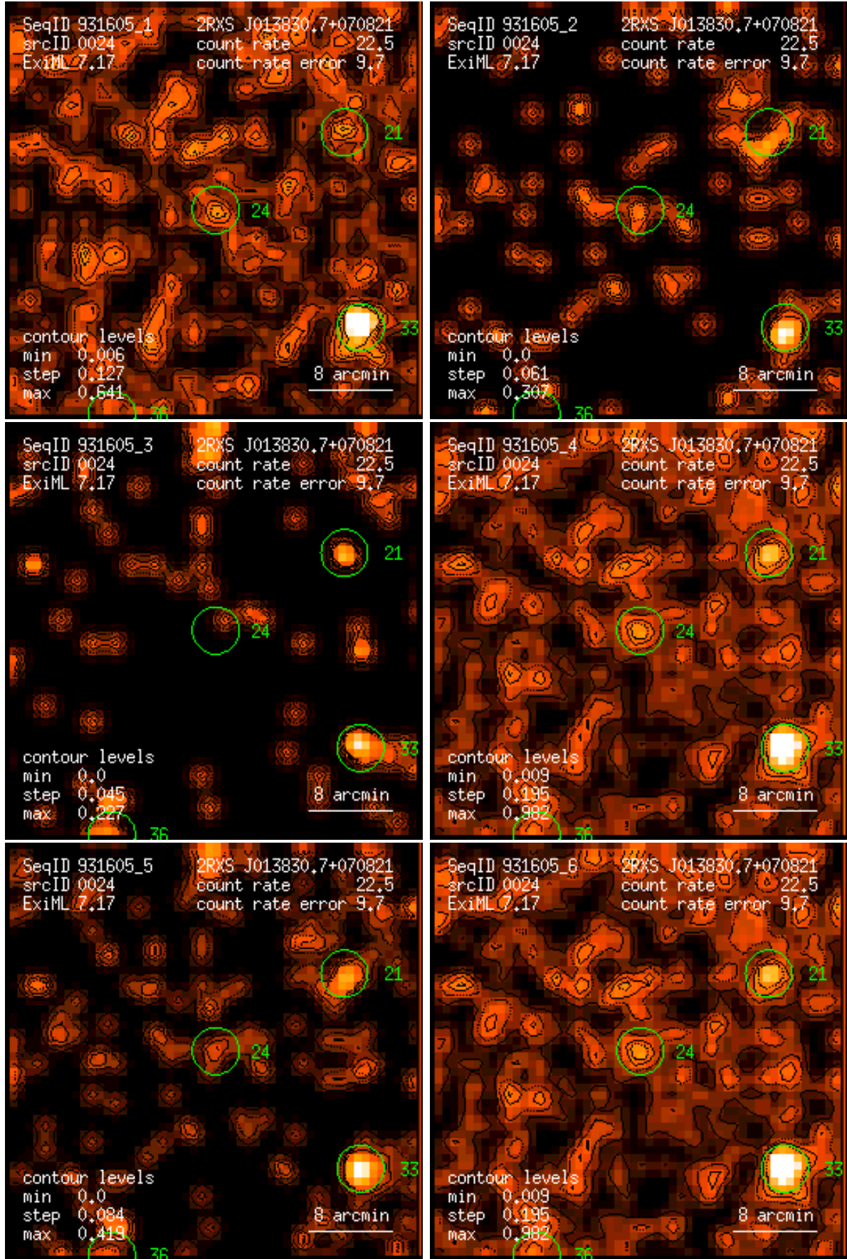
Figure 24: RASS 931605: detection 0024: band rate images, Gaussian filter: (1) PSPC channels 11 – 41, (2) 52 – 90, (3) 91 – 201, (4) 11 – 235, (5) 52 – 201, (6) 11 – 201. Broad band rates in counts/ks. Band rate contour levels in counts/ks/arcmin 2 .
