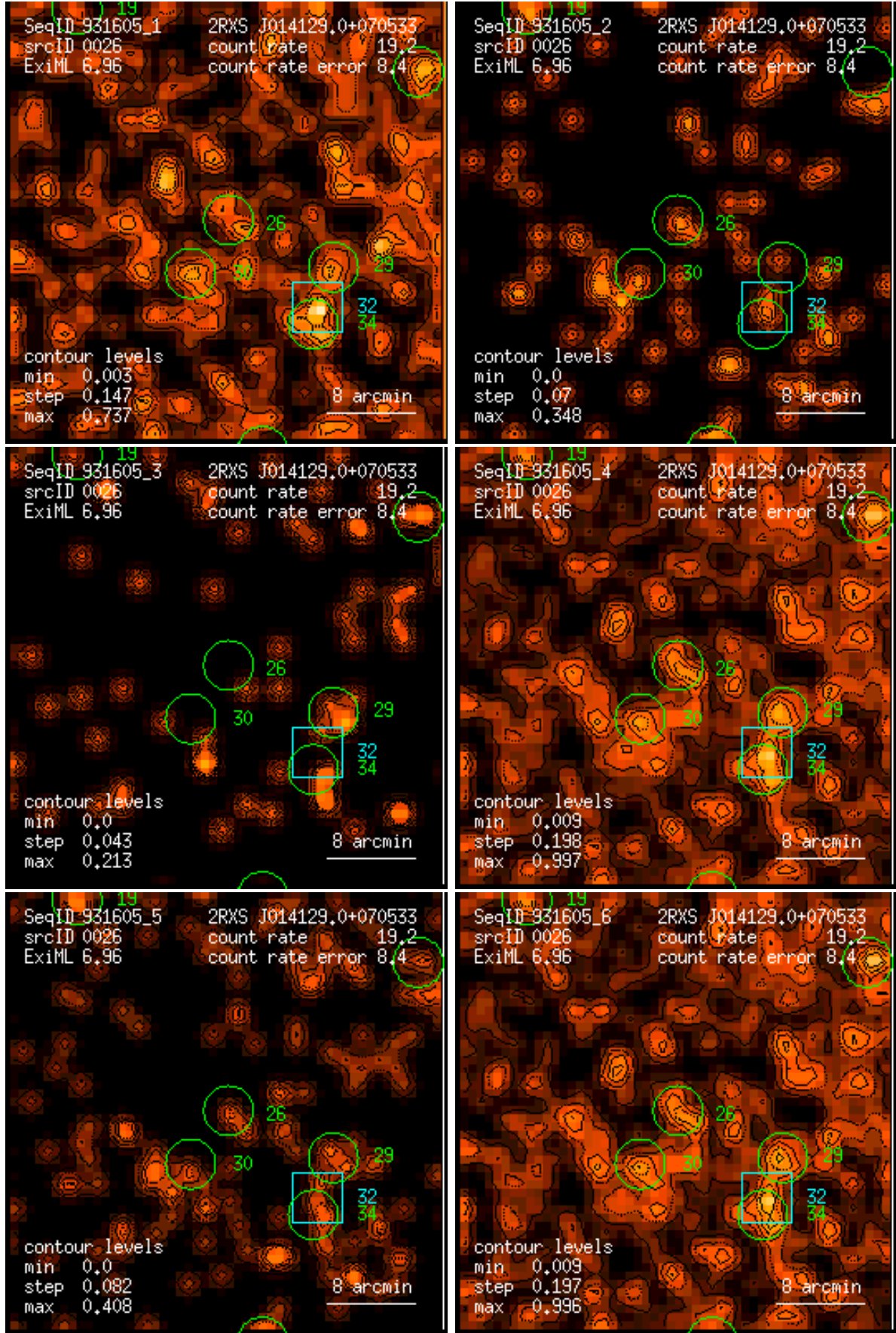
Figure 26: RASS 931605: detection 0026: band rate images, Gaussian filter: (1) PSPC channels 11 – 41, (2) 52 – 90, (3) 91 – 201, (4) 11 – 235, (5) 52 – 201, (6) 11 – 201. Broad band rates in counts/ks. Band rate contour levels in counts/ks/arcmin 2 .
