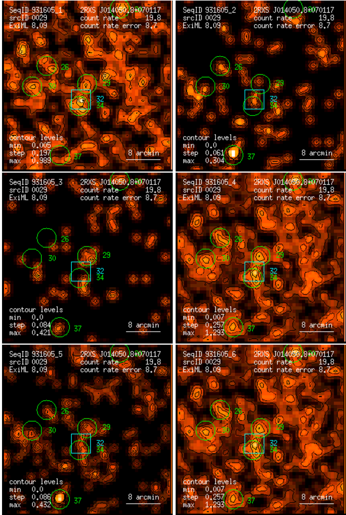
Figure 29: RASS 931605: detection 0029: band rate images, Gaussian filter: (1) PSPC channels 11 – 41, (2) 52 – 90, (3) 91 – 201, (4) 11 – 235, (5) 52 – 201, (6) 11 – 201. Broad band rates in counts/ks. Band rate contour levels in counts/ks/arcmin 2 .
