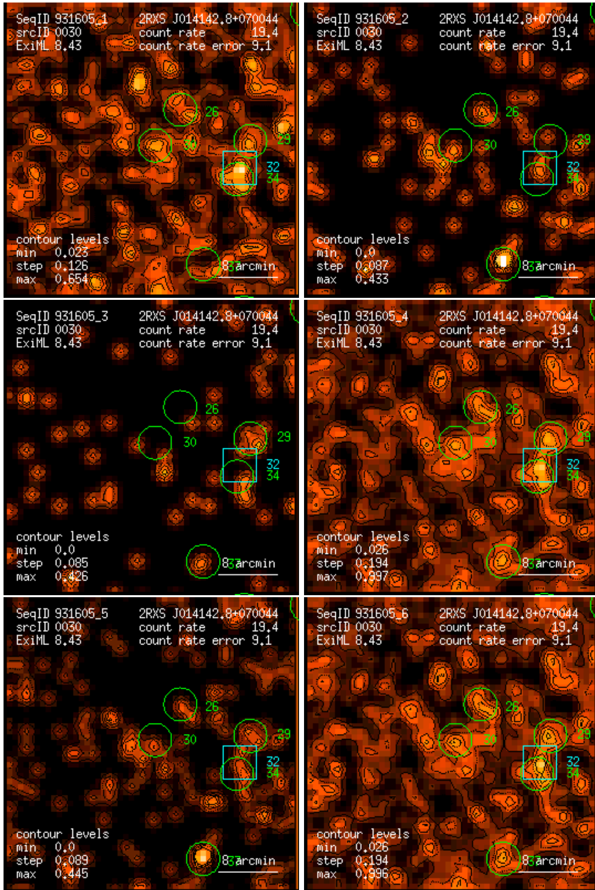
Figure 30: RASS 931605: detection 0030: band rate images, Gaussian filter: (1) PSPC channels 11 – 41, (2) 52 – 90, (3) 91 – 201, (4) 11 – 235, (5) 52 – 201, (6) 11 – 201. Broad band rates in counts/ks. Band rate contour levels in counts/ks/arcmin 2 .
