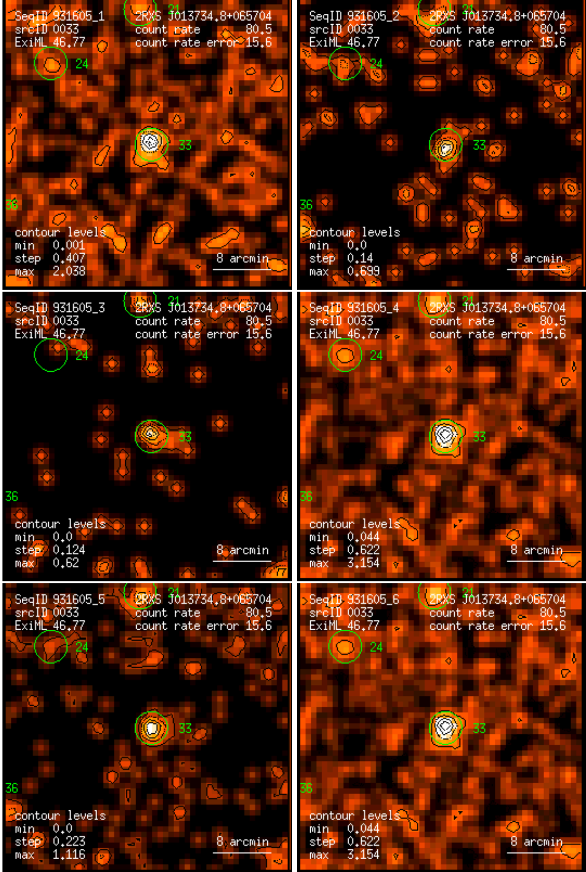
Figure 33: RASS 931605: detection 0033: band rate images, Gaussian filter: (1) PSPC channels 11 – 41, (2) 52 – 90, (3) 91 – 201, (4) 11 – 235, (5) 52 – 201, (6) 11 – 201. Broad band rates in counts/ks. Band rate contour levels in counts/ks/arcmin 2 .
