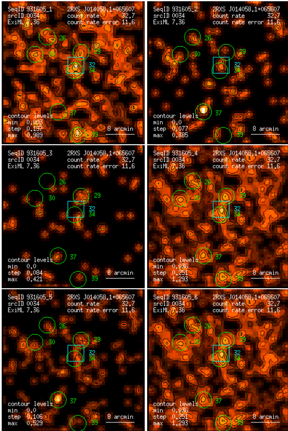
Figure 34: RASS 931605: detection 0034: band rate images, Gaussian filter: (1) PSPC channels 11 – 41, (2) 52 – 90, (3) 91 – 201, (4) 11 – 235, (5) 52 – 201, (6) 11 – 201. Broad band rates in counts/ks. Band rate contour levels in counts/ks/arcmin 2 .
