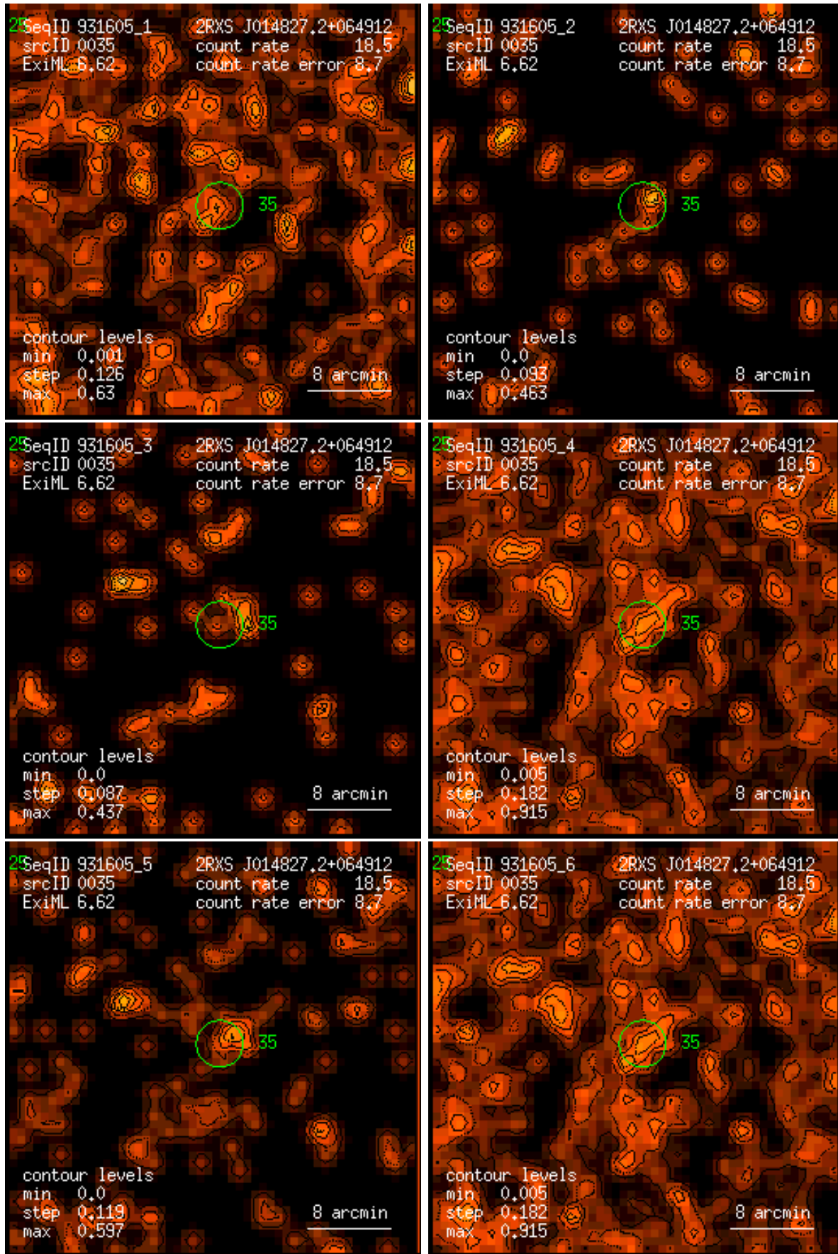
Figure 35: RASS 931605: detection 0035: band rate images, Gaussian filter: (1) PSPC channels 11 – 41, (2) 52 – 90, (3) 91 – 201, (4) 11 – 235, (5) 52 – 201, (6) 11 – 201. Broad band rates in counts/ks. Band rate contour levels in counts/ks/arcmin 2 .
