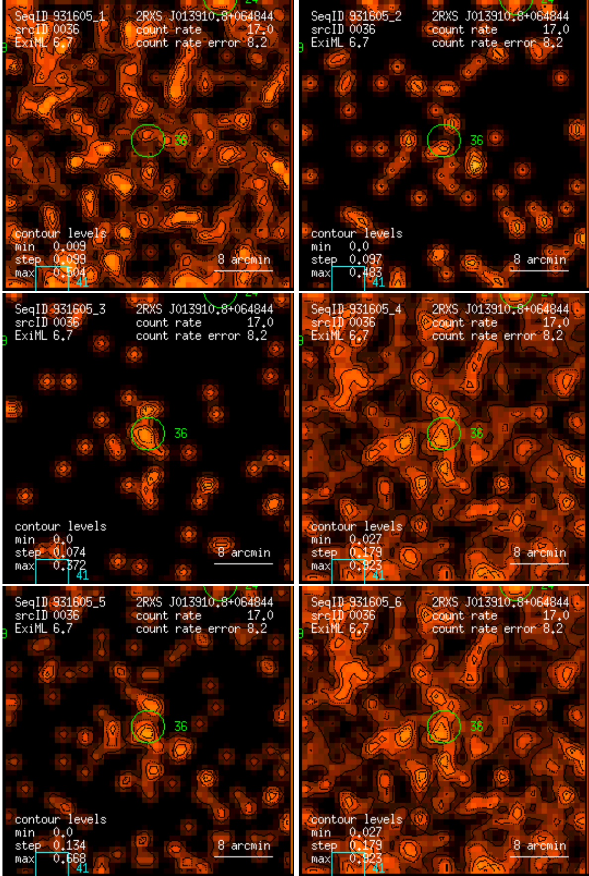
Figure 36: RASS 931605: detection 0036: band rate images, Gaussian filter: (1) PSPC channels 11 – 41, (2) 52 – 90, (3) 91 – 201, (4) 11 – 235, (5) 52 – 201, (6) 11 – 201. Broad band rates in counts/ks. Band rate contour levels in counts/ks/arcmin 2 .
