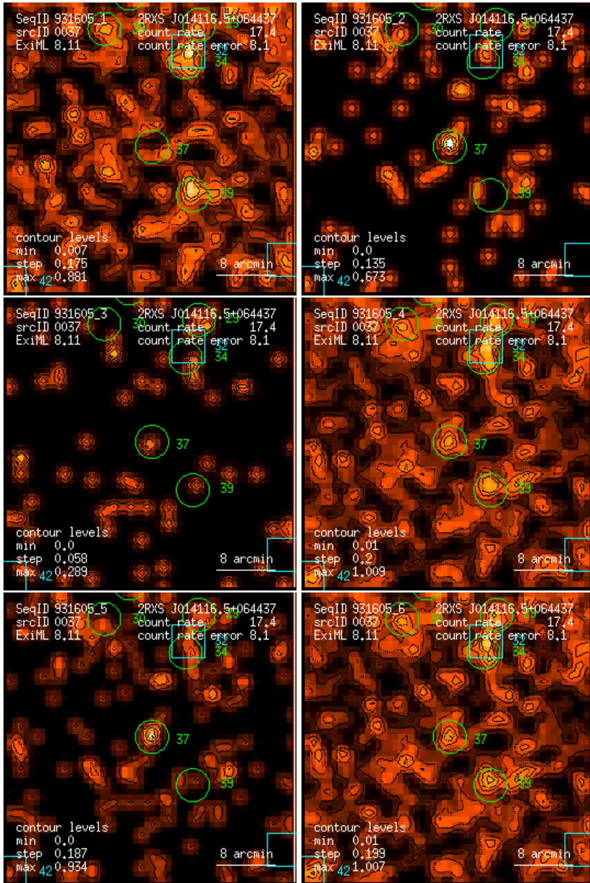
Figure 37: RASS 931605: detection 0037: band rate images, Gaussian filter: (1) PSPC channels 11 – 41, (2) 52 – 90, (3) 91 – 201, (4) 11 – 235, (5) 52 – 201, (6) 11 – 201. Broad band rates in counts/ks. Band rate contour levels in counts/ks/arcmin 2 .
