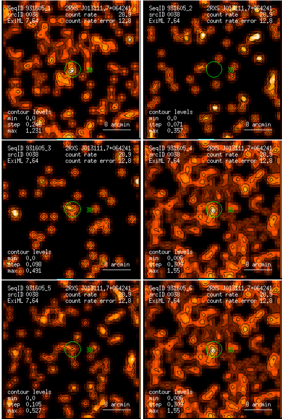
Figure 38: RASS 931605: detection 0038: band rate images, Gaussian filter: (1) PSPC channels 11 – 41, (2) 52 – 90, (3) 91 – 201, (4) 11 – 235, (5) 52 – 201, (6) 11 – 201. Broad band rates in counts/ks. Band rate contour levels in counts/ks/arcmin 2 .
