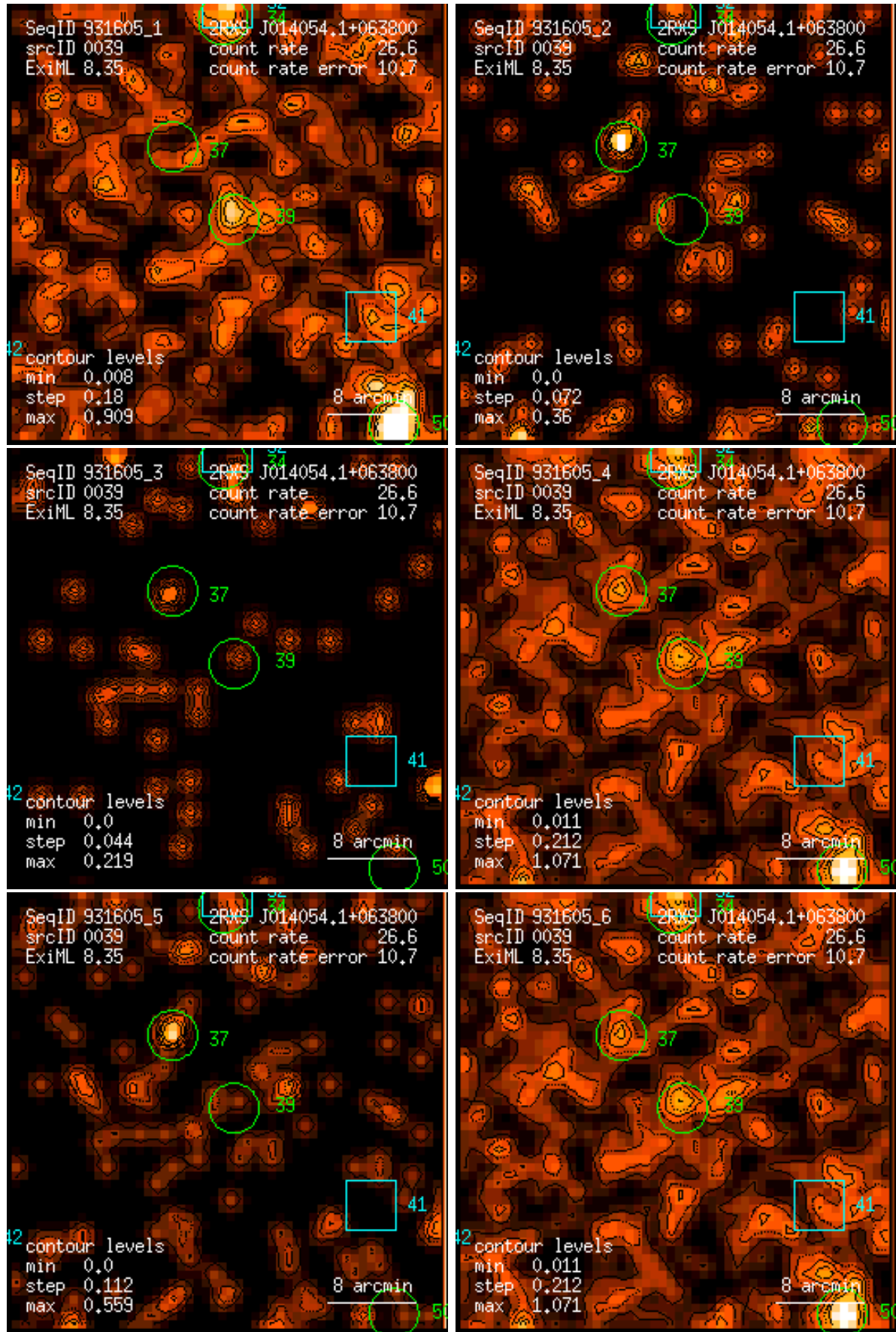
Figure 39: RASS 931605: detection 0039: band rate images, Gaussian filter: (1) PSPC channels 11 – 41, (2) 52 – 90, (3) 91 – 201, (4) 11 – 235, (5) 52 – 201, (6) 11 – 201. Broad band rates in counts/ks. Band rate contour levels in counts/ks/arcmin 2 .
