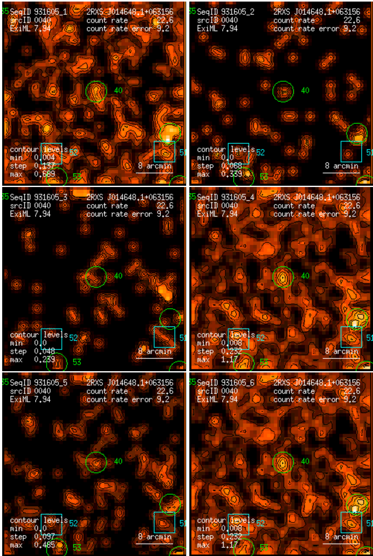
Figure 40: RASS 931605: detection 0040: band rate images, Gaussian filter: (1) PSPC channels 11 – 41, (2) 52 – 90, (3) 91 – 201, (4) 11 – 235, (5) 52 – 201, (6) 11 – 201. Broad band rates in counts/ks. Band rate contour levels in counts/ks/arcmin 2 .
