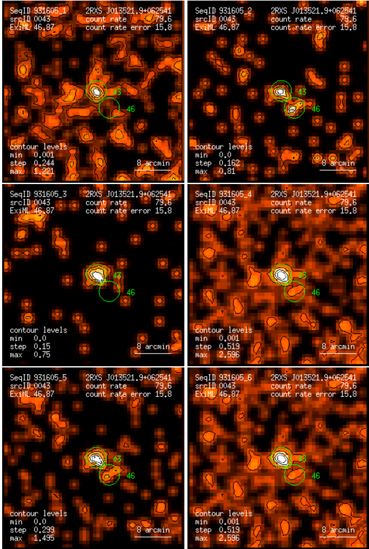
Figure 43: RASS 931605: detection 0043: band rate images, Gaussian filter: (1) PSPC channels 11 – 41, (2) 52 – 90, (3) 91 – 201, (4) 11 – 235, (5) 52 – 201, (6) 11 – 201. Broad band rates in counts/ks. Band rate contour levels in counts/ks/arcmin 2 .
