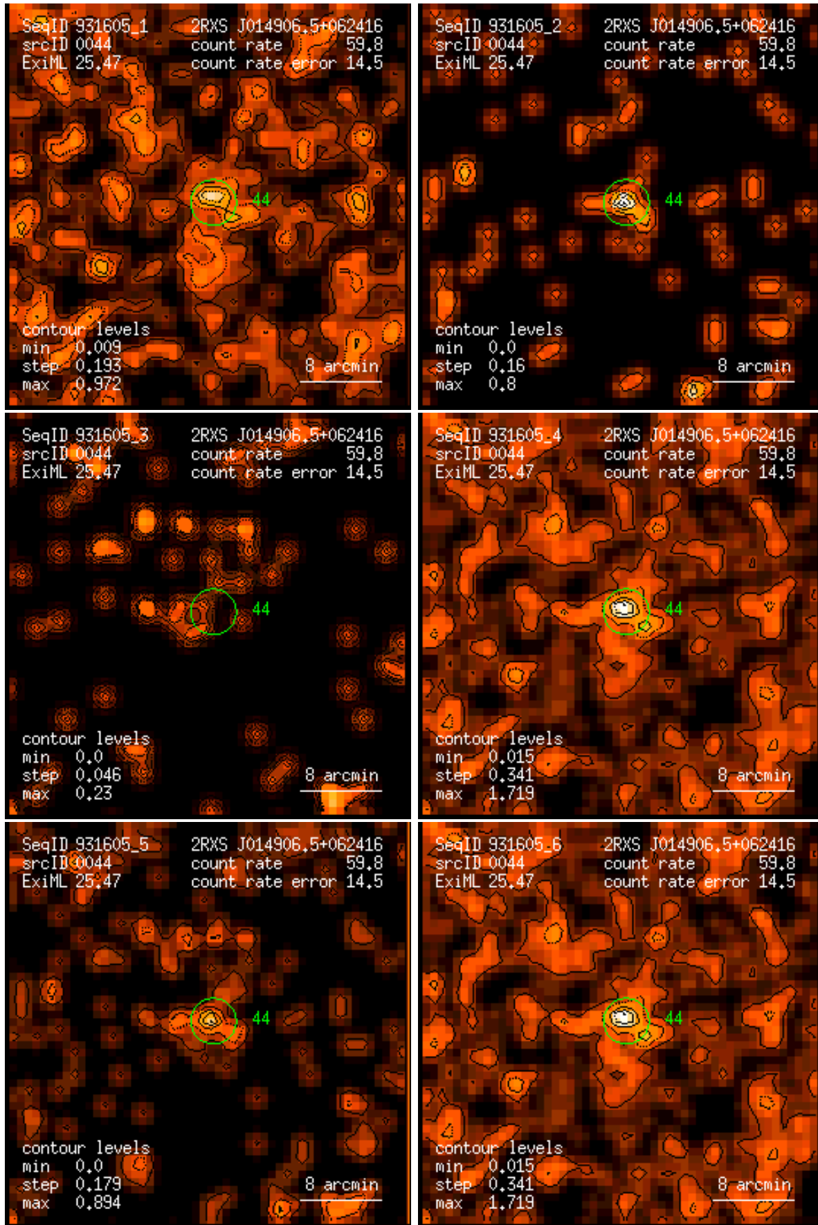
Figure 44: RASS 931605: detection 0044: band rate images, Gaussian filter: (1) PSPC channels 11 – 41, (2) 52 – 90, (3) 91 – 201, (4) 11 – 235, (5) 52 – 201, (6) 11 – 201. Broad band rates in counts/ks. Band rate contour levels in counts/ks/arcmin 2 .
