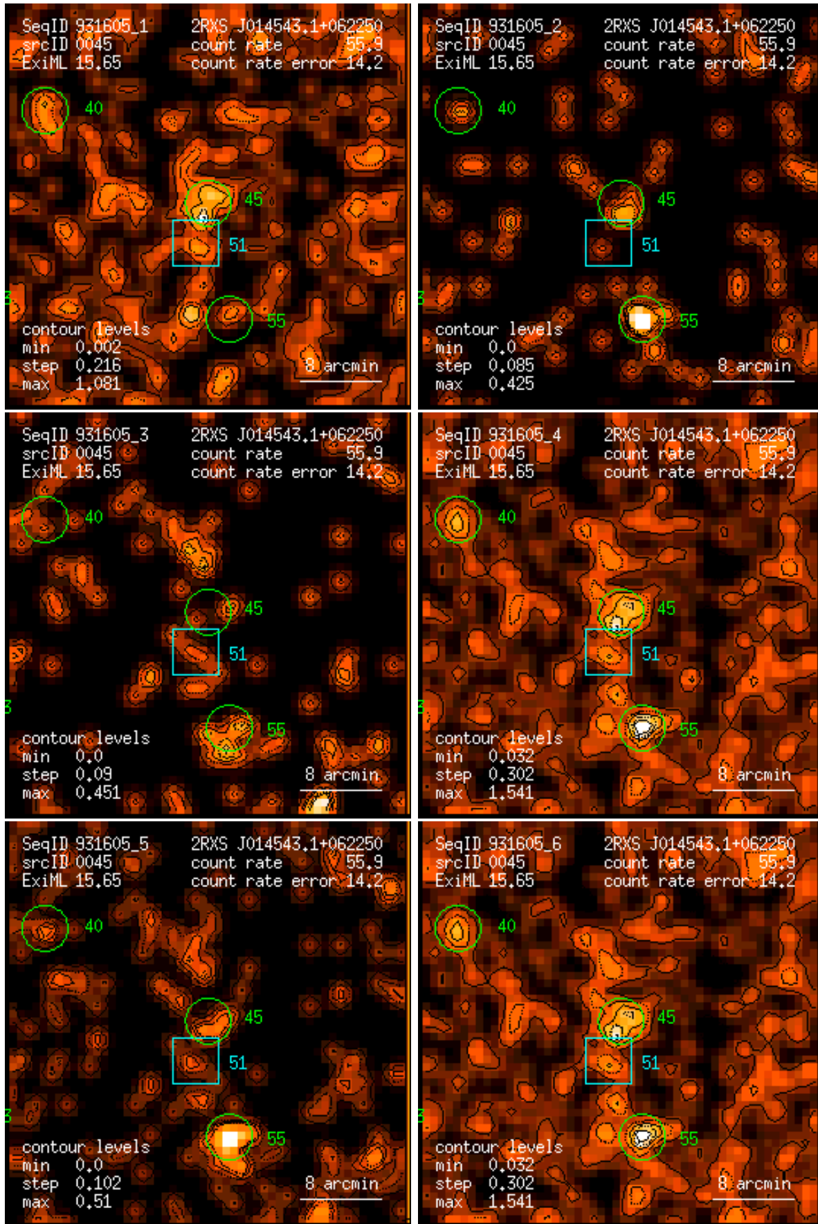
Figure 45: RASS 931605: detection 0045: band rate images, Gaussian filter: (1) PSPC channels 11 – 41, (2) 52 – 90, (3) 91 – 201, (4) 11 – 235, (5) 52 – 201, (6) 11 – 201. Broad band rates in counts/ks. Band rate contour levels in counts/ks/arcmin 2 .
