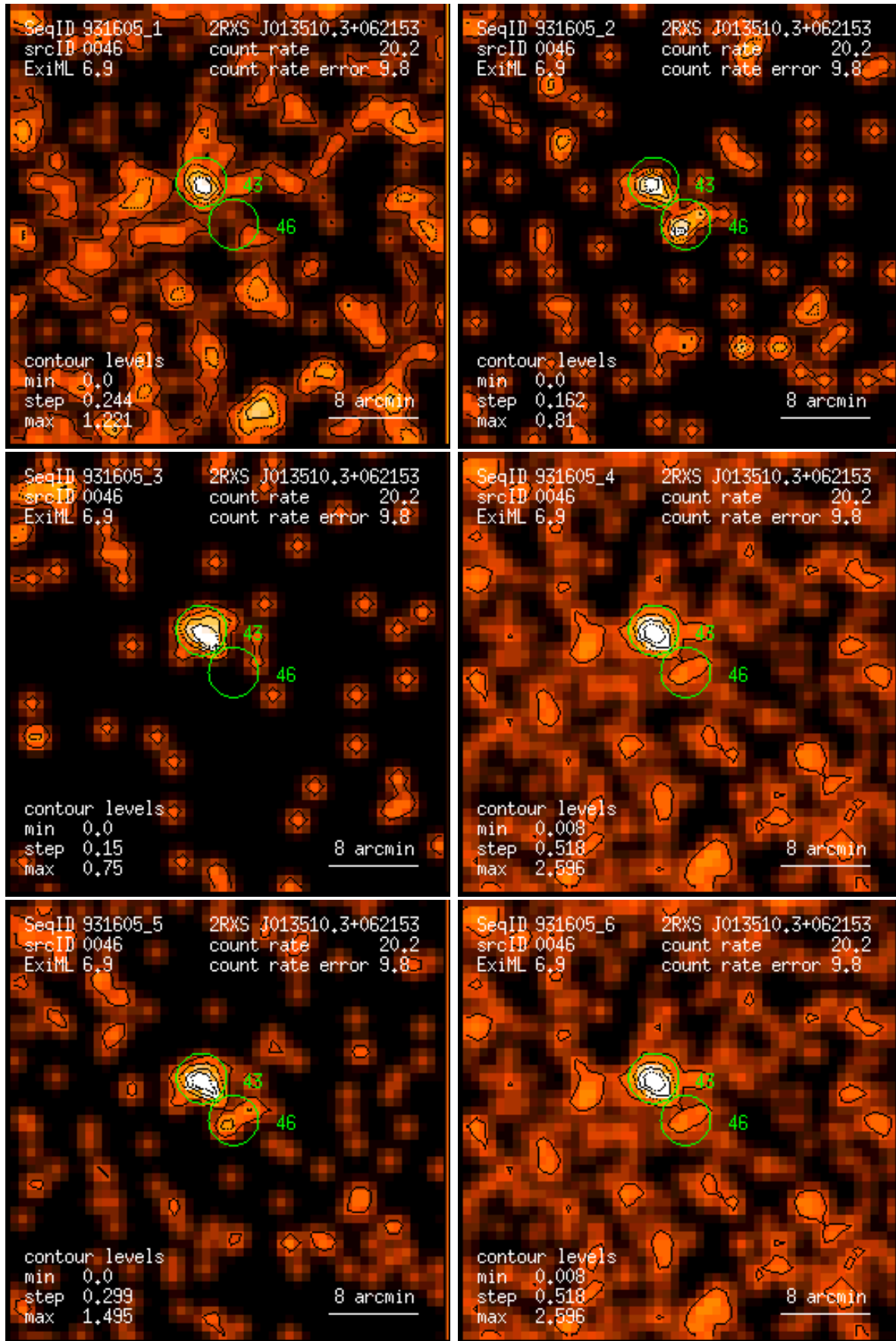
Figure 46: RASS 931605: detection 0046: band rate images, Gaussian filter: (1) PSPC channels 11 – 41, (2) 52 – 90, (3) 91 – 201, (4) 11 – 235, (5) 52 – 201, (6) 11 – 201. Broad band rates in counts/ks. Band rate contour levels in counts/ks/arcmin 2 .
