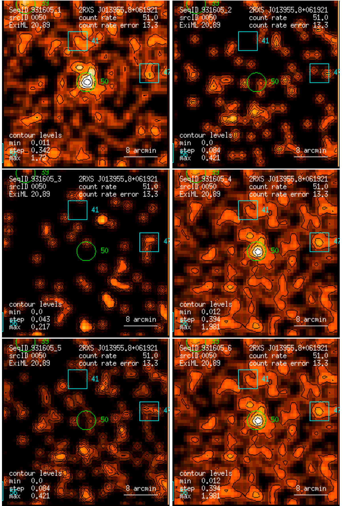
Figure 50: RASS 931605: detection 0050: band rate images, Gaussian filter: (1) PSPC channels 11 – 41, (2) 52 – 90, (3) 91 – 201, (4) 11 – 235, (5) 52 – 201, (6) 11 – 201. Broad band rates in counts/ks. Band rate contour levels in counts/ks/arcmin 2 .
