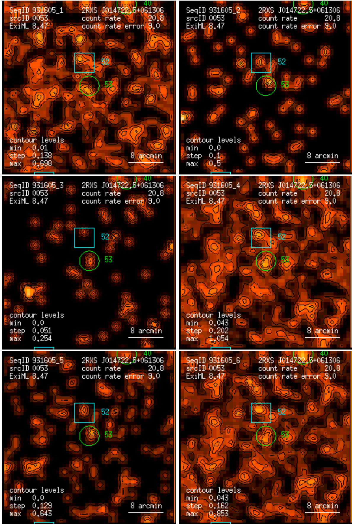
Figure 53: RASS 931605: detection 0053: band rate images, Gaussian filter: (1) PSPC channels 11 – 41, (2) 52 – 90, (3) 91 – 201, (4) 11 – 235, (5) 52 – 201, (6) 11 – 201. Broad band rates in counts/ks. Band rate contour levels in counts/ks/arcmin 2 .
