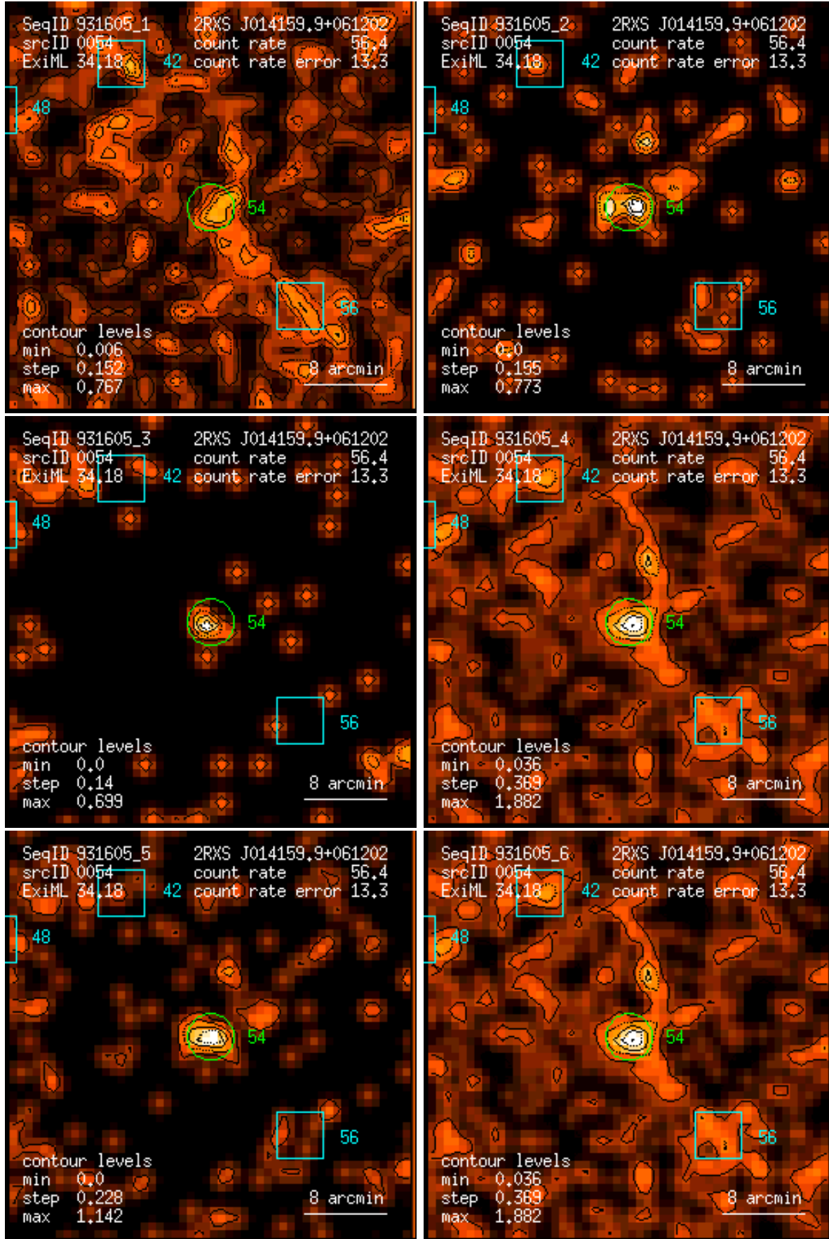
Figure 54: RASS 931605: detection 0054: band rate images, Gaussian filter: (1) PSPC channels 11 – 41, (2) 52 – 90, (3) 91 – 201, (4) 11 – 235, (5) 52 – 201, (6) 11 – 201. Broad band rates in counts/ks. Band rate contour levels in counts/ks/arcmin 2 .
