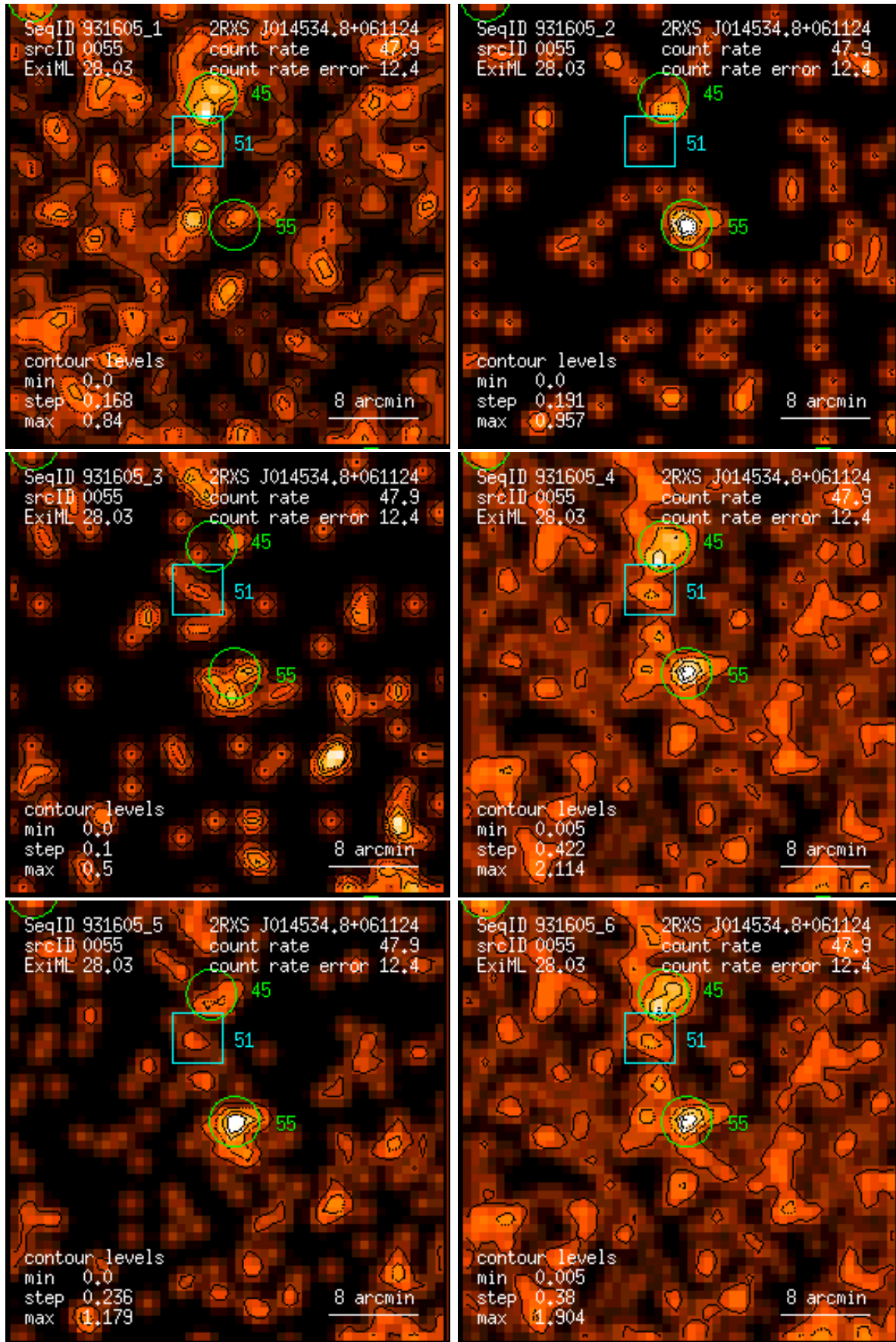
Figure 55: RASS 931605: detection 0055: band rate images, Gaussian filter: (1) PSPC channels 11 – 41, (2) 52 – 90, (3) 91 – 201, (4) 11 – 235, (5) 52 – 201, (6) 11 – 201. Broad band rates in counts/ks. Band rate contour levels in counts/ks/arcmin 2 .
