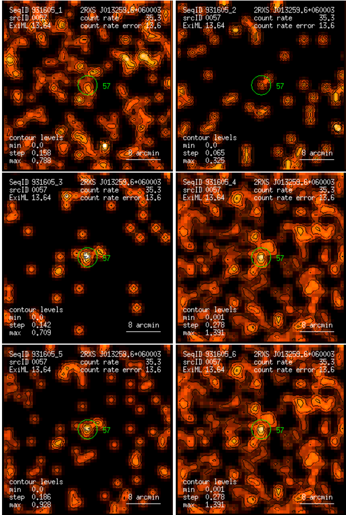
Figure 57: RASS 931605: detection 0057: band rate images, Gaussian filter: (1) PSPC channels 11 – 41, (2) 52 – 90, (3) 91 – 201, (4) 11 – 235, (5) 52 – 201, (6) 11 – 201. Broad band rates in counts/ks. Band rate contour levels in counts/ks/arcmin 2 .
