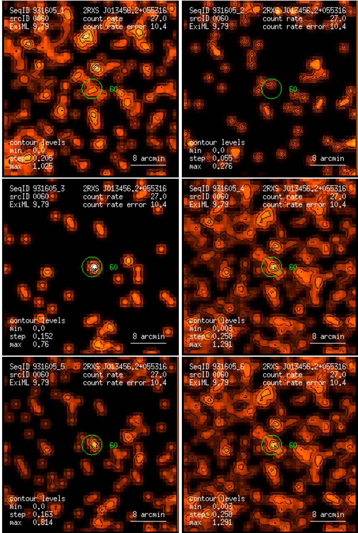
Figure 60: RASS 931605: detection 0060: band rate images, Gaussian filter: (1) PSPC channels 11 – 41, (2) 52 – 90, (3) 91 – 201, (4) 11 – 235, (5) 52 – 201, (6) 11 – 201. Broad band rates in counts/ks. Band rate contour levels in counts/ks/arcmin 2 .
