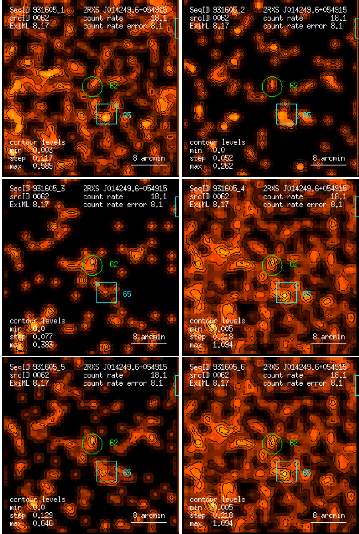
Figure 62: RASS 931605: detection 0062: band rate images, Gaussian filter: (1) PSPC channels 11 – 41, (2) 52 – 90, (3) 91 – 201, (4) 11 – 235, (5) 52 – 201, (6) 11 – 201. Broad band rates in counts/ks. Band rate contour levels in counts/ks/arcmin 2 .
