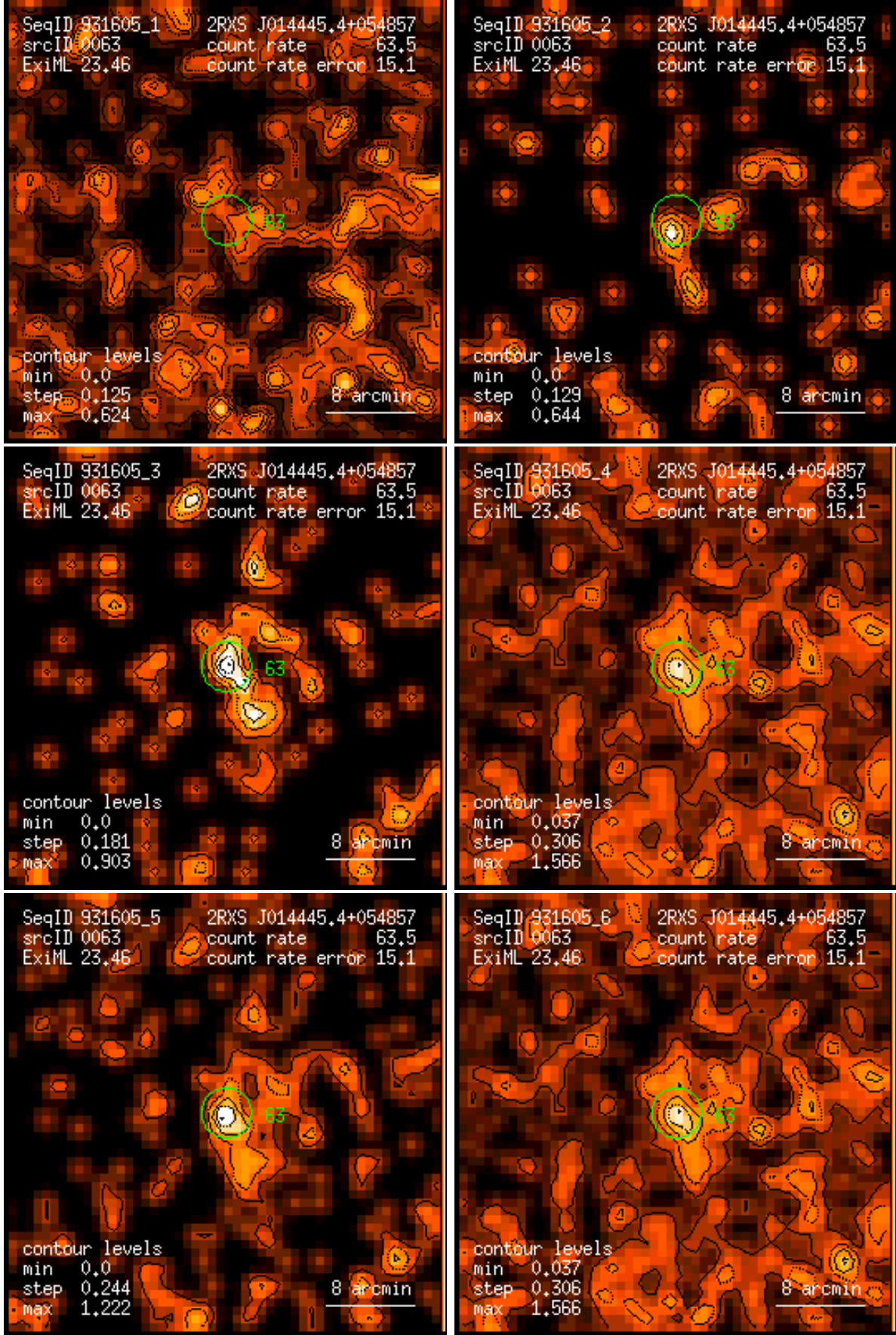
Figure 63: RASS 931605: detection 0063: band rate images, Gaussian filter: (1) PSPC channels 11 – 41, (2) 52 – 90, (3) 91 – 201, (4) 11 – 235, (5) 52 – 201, (6) 11 – 201. Broad band rates in counts/ks. Band rate contour levels in counts/ks/arcmin 2 .
