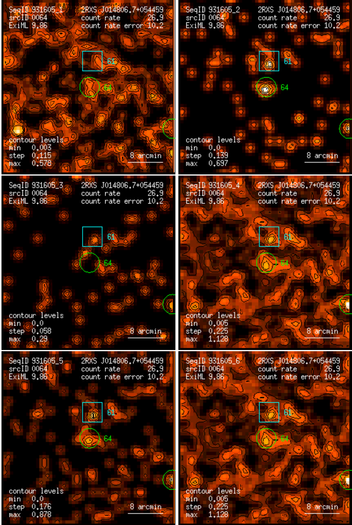
Figure 64: RASS 931605: detection 0064: band rate images, Gaussian filter: (1) PSPC channels 11 – 41, (2) 52 – 90, (3) 91 – 201, (4) 11 – 235, (5) 52 – 201, (6) 11 – 201. Broad band rates in counts/ks. Band rate contour levels in counts/ks/arcmin 2 .
