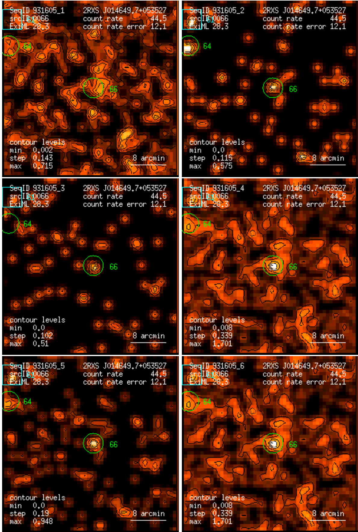
Figure 66: RASS 931605: detection 0066: band rate images, Gaussian filter: (1) PSPC channels 11 – 41, (2) 52 – 90, (3) 91 – 201, (4) 11 – 235, (5) 52 – 201, (6) 11 – 201. Broad band rates in counts/ks. Band rate contour levels in counts/ks/arcmin 2 .
