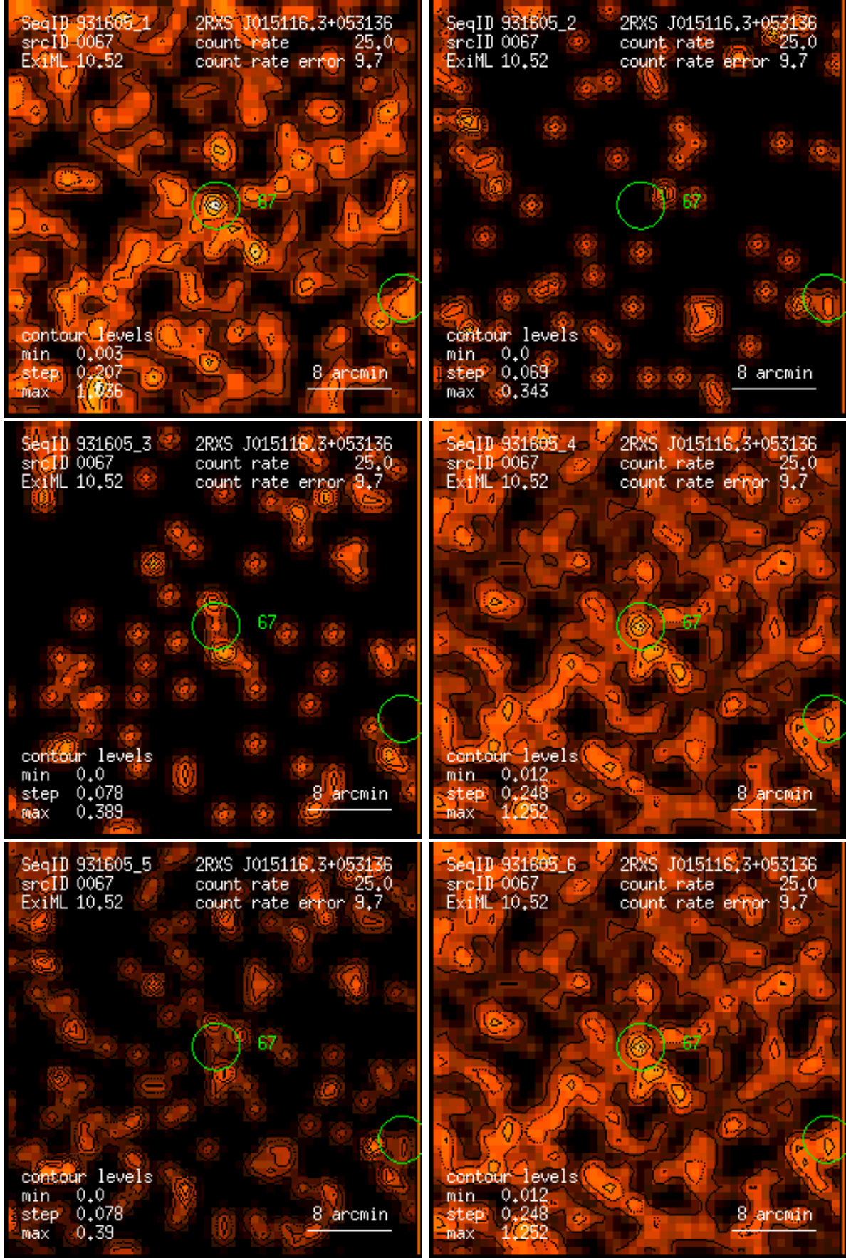
Figure 67: RASS 931605: detection 0067: band rate images, Gaussian filter: (1) PSPC channels 11 – 41, (2) 52 – 90, (3) 91 – 201, (4) 11 – 235, (5) 52 – 201, (6) 11 – 201. Broad band rates in counts/ks. Band rate contour levels in counts/ks/arcmin 2 .
